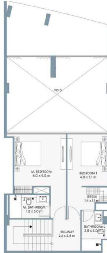
MEZZANINE
