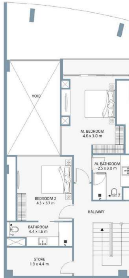
MEZZANINE
